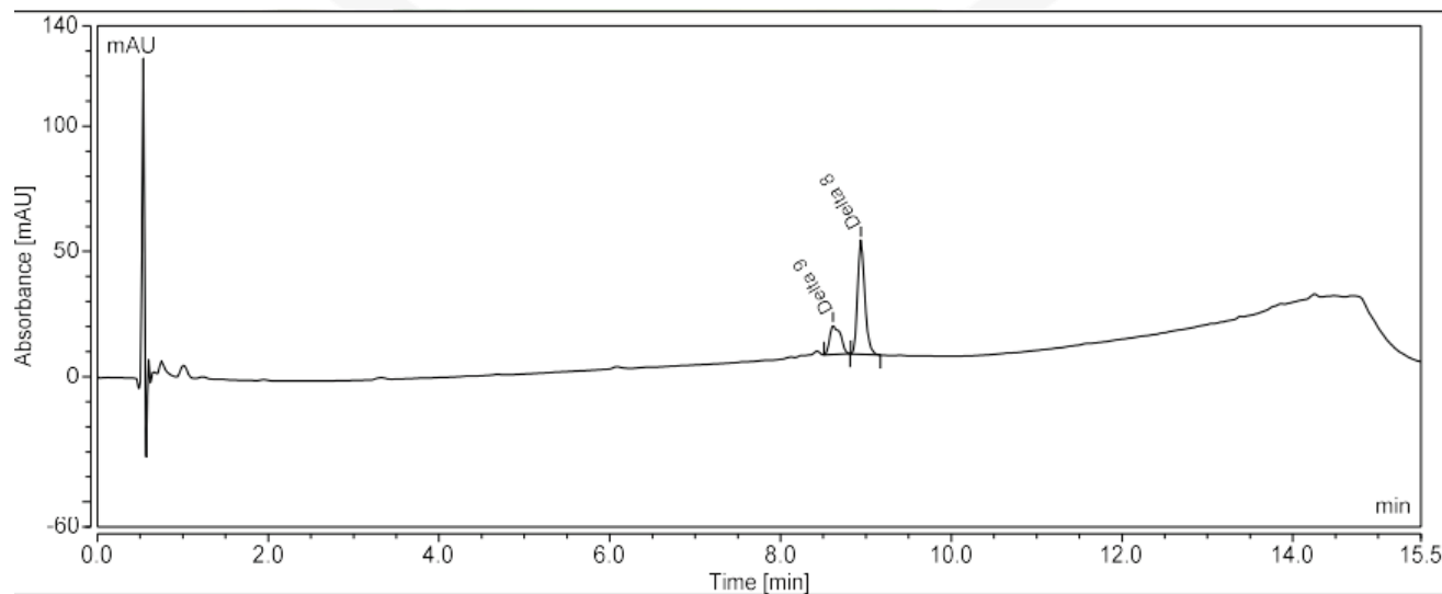
CROMATOGRAMA [MC062022-005]
