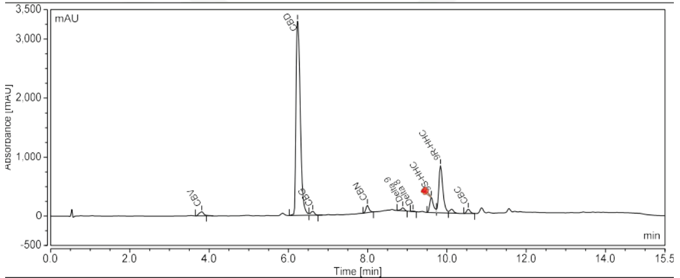
CROMATOGRAMA [MC082022-027]
