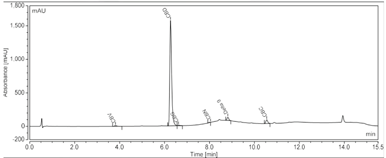
CROMATOGRAMA [MC082022-028]
