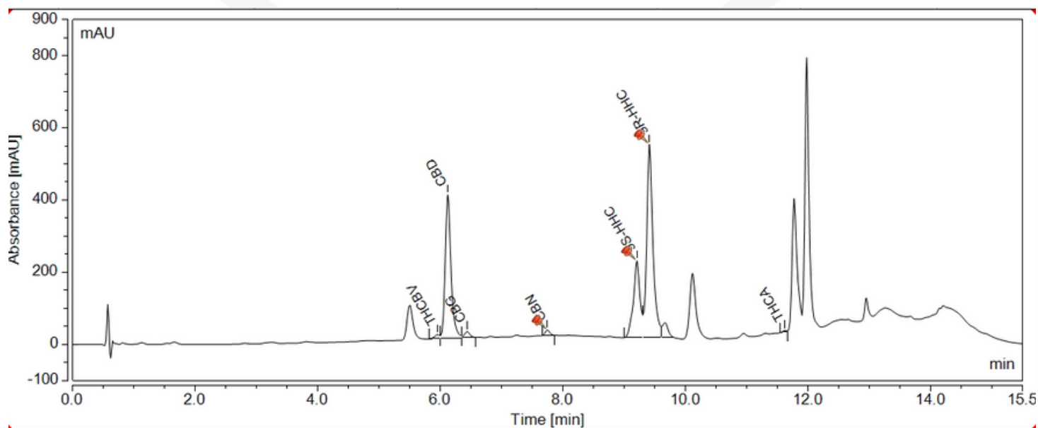
CROMATOGRAMA [MC052023-069]
