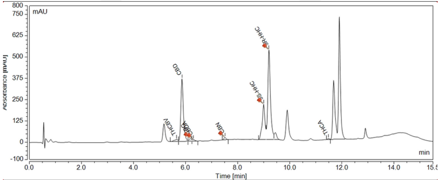
CROMATOGRAMA [MC052023-073]
