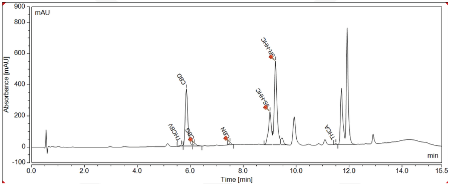
CROMATOGRAMA [MC052023-078]
